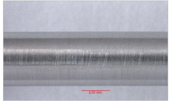
UR™ 4565 after 720 hours (7 bar H 2 S, 250 g/l NaCl, pH 4.5, 150 °C) at 90%AYS
