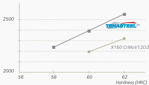
Compression strength R(0.2) MPa
