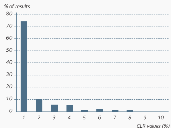
HISTOGRAM OF TYPICAL VALUES FROM HIC TESTING ON INDUSTRIAL PRODUCTION
