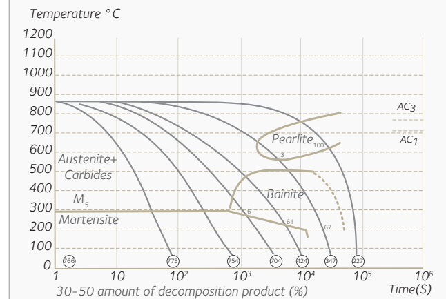
CT DIAGRAM AUSTENITIZING TEMPERATURE 850°C - O-HARDNESS, HV
