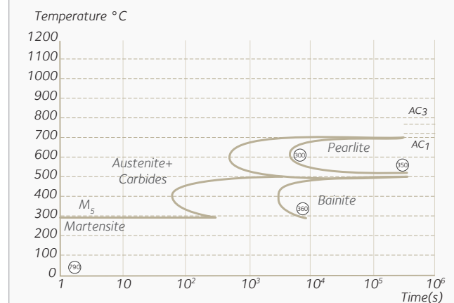
TTT DIAGRAM AUSTENITIZING TEMPERATURE 850°C - O-HARDNESS, HV
